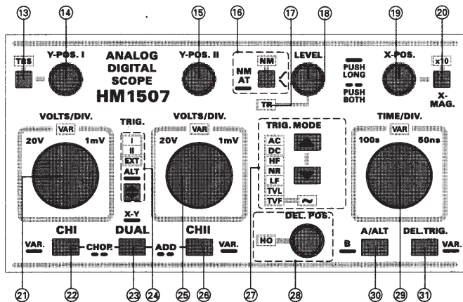
(25) VOLTS/DIV. – Control knob
